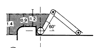
④ Control trap with draining base
